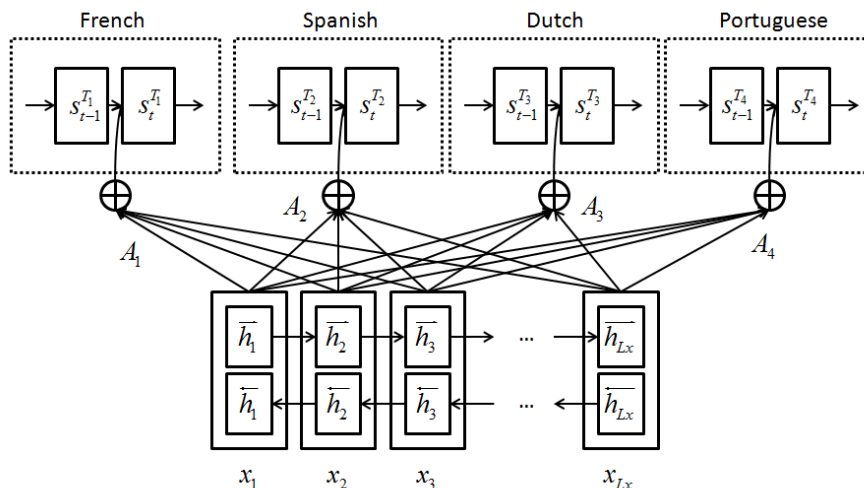
Figure 2: Multi-task learning framework for multiple-target language translation
