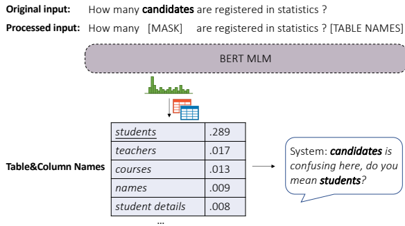
Figure 5: Token Correction in PHOTON.
