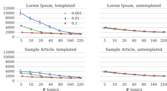
Figure 6: LDA training perplexity for REUSL 2.5k with different types of templated text repetition. The effect of duplication is prominent for small numbers of topics but diminishes with more topics to sufficiently model the missing text. With the fraction of the corpus that contains duplicates p = 0.1 , the perplexity of template documents is below that of untemplated texts.
