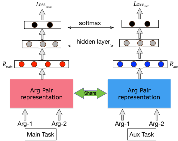
Figure 3: The framework of our proposed multi-task attention-based neural network model.
