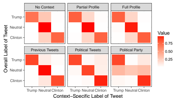
Figure 2: Parameter matrices \gamma^c learned by ConStance for each context. Darker shading indicates higher values.
